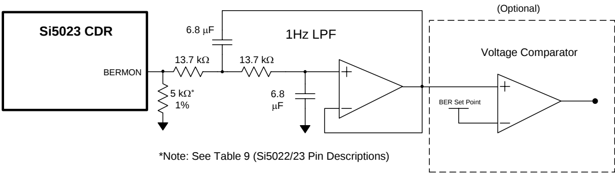
Figure 9. Si5023 BERMON Application Schematic
